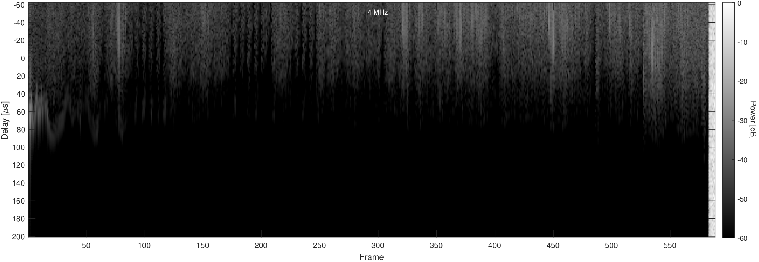
Orbit 21075, Chapman, No Window, Channel 2
