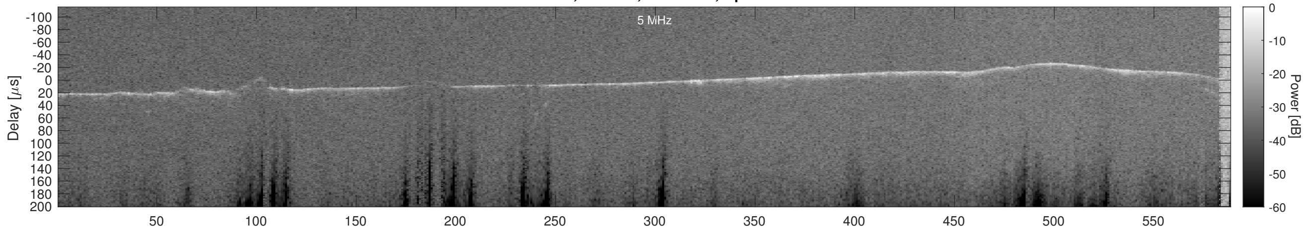
Orbit 21075, Cluttergram
