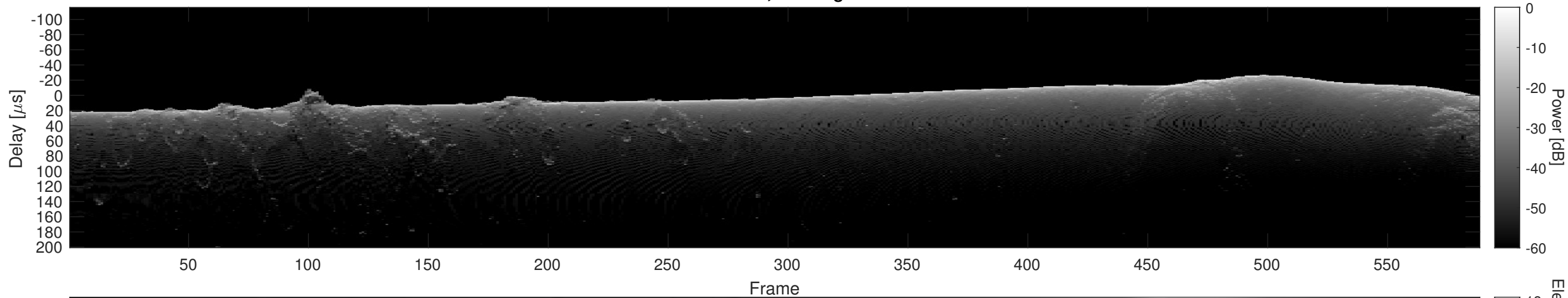
Orbit 21075, Cluttergram
