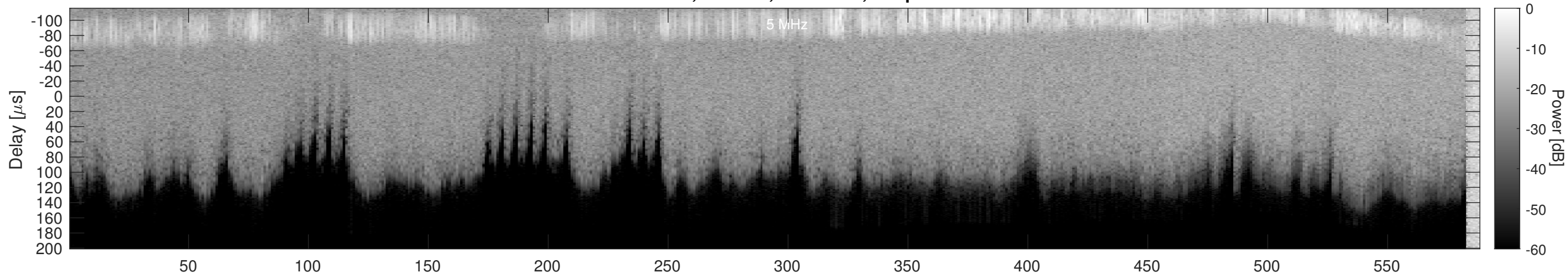
Orbit 21075, Window, Channel 1, Optimized
