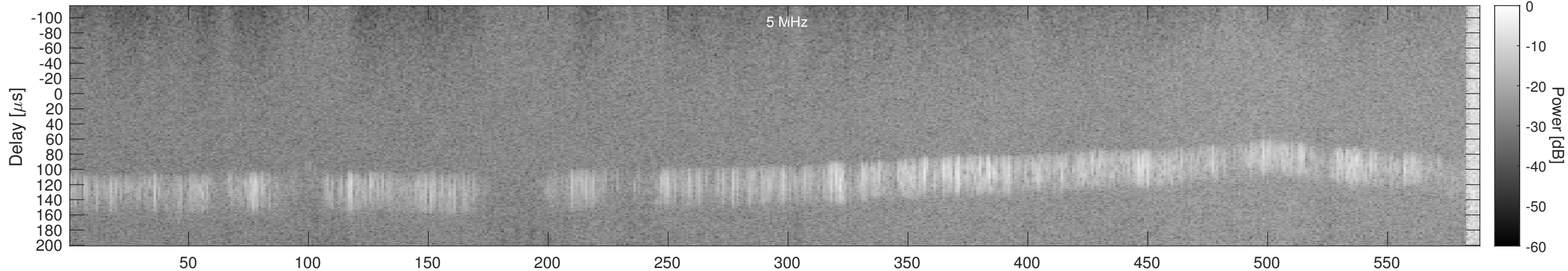
Orbit 21075, Window, Channel 1, Chapman
