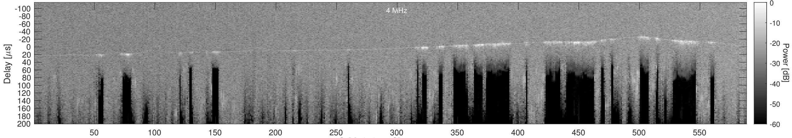
Orbit 21075, Cluttergram
