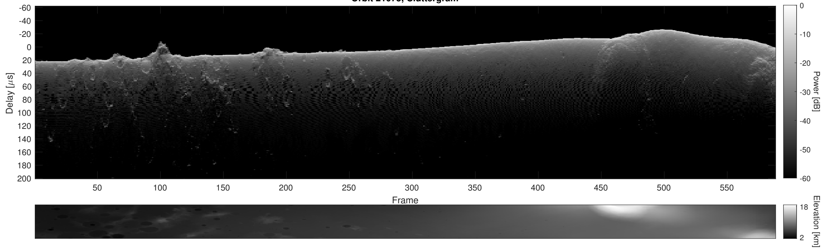
Orbit 21075, Cluttergram
