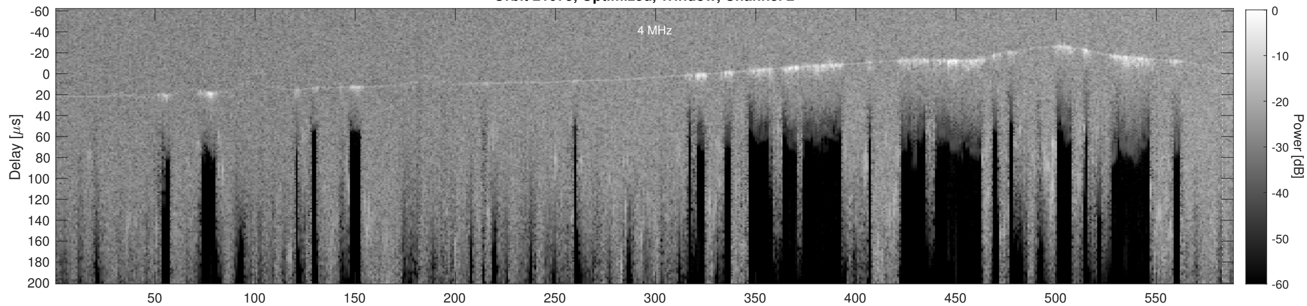
Orbit 21075, Cluttergram
