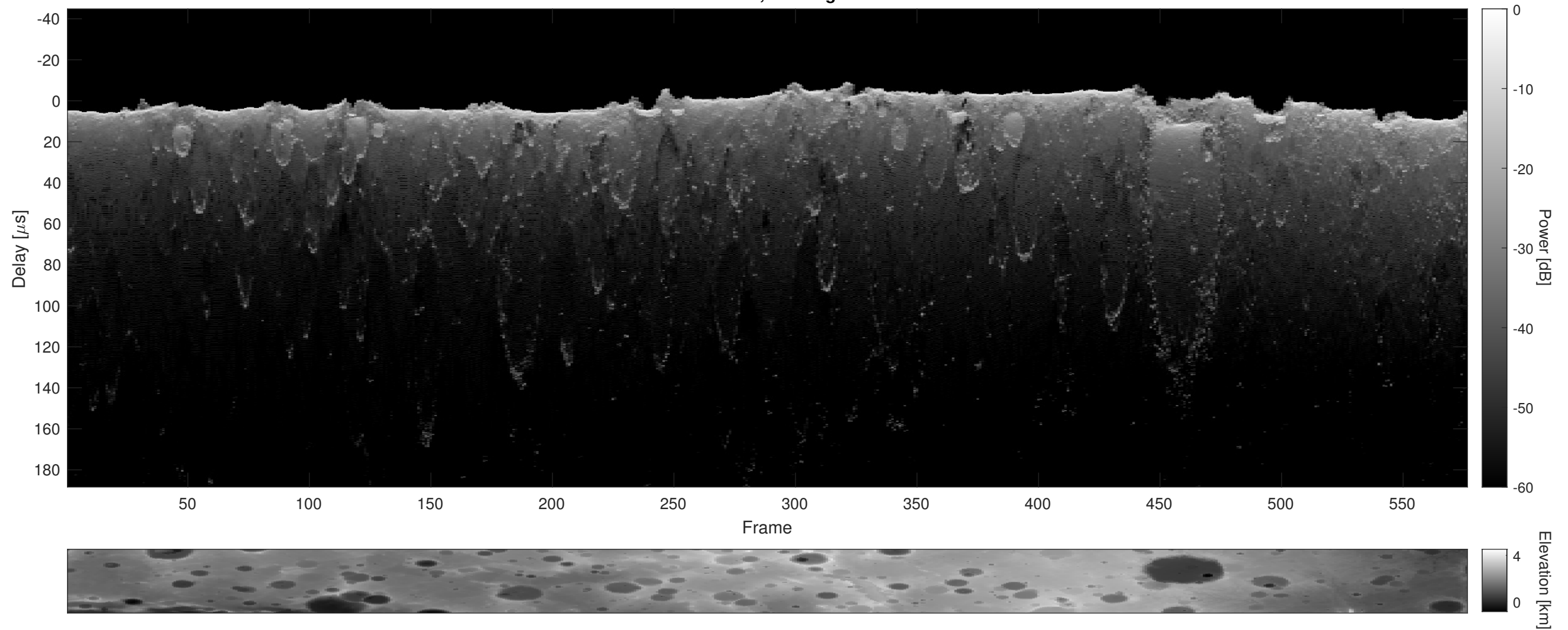
Orbit 21077, Cluttergram
