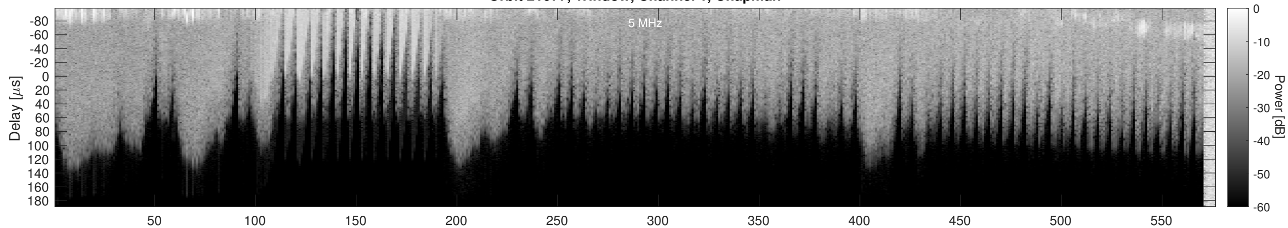
Orbit 21077, Window, Channel 1, Optimized
