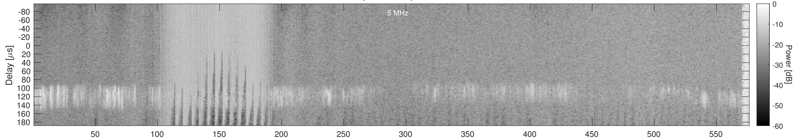
Orbit 21077, Window, Channel 1, Chapman
