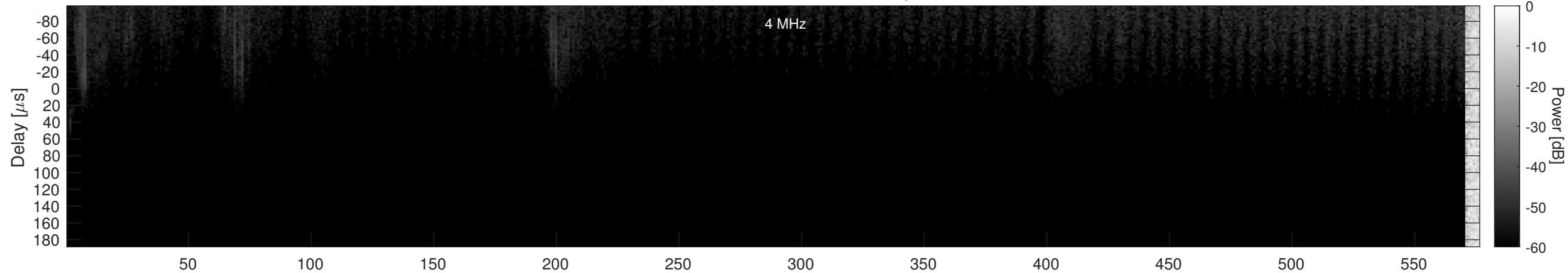
Orbit 21077, Window, Channel 2, Optimized
