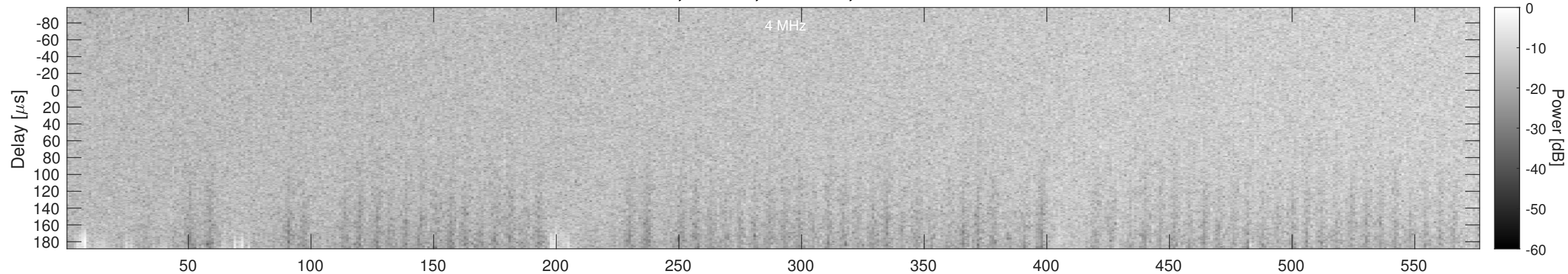
Orbit 21077, Window, Channel 2, Chapman
