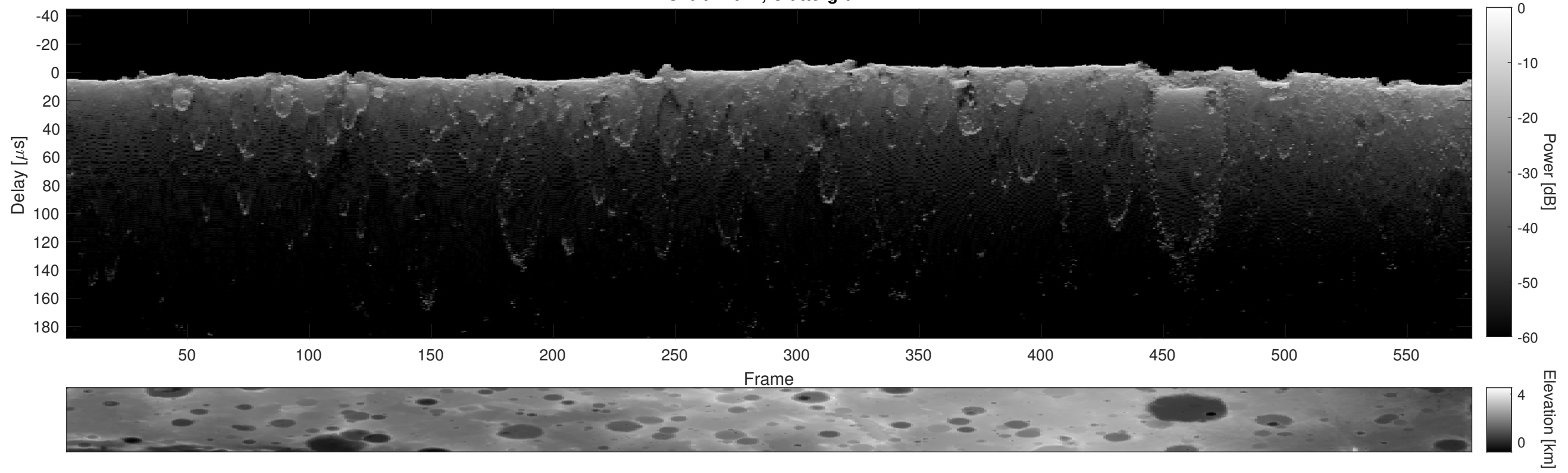
Orbit 21077, Cluttergram
