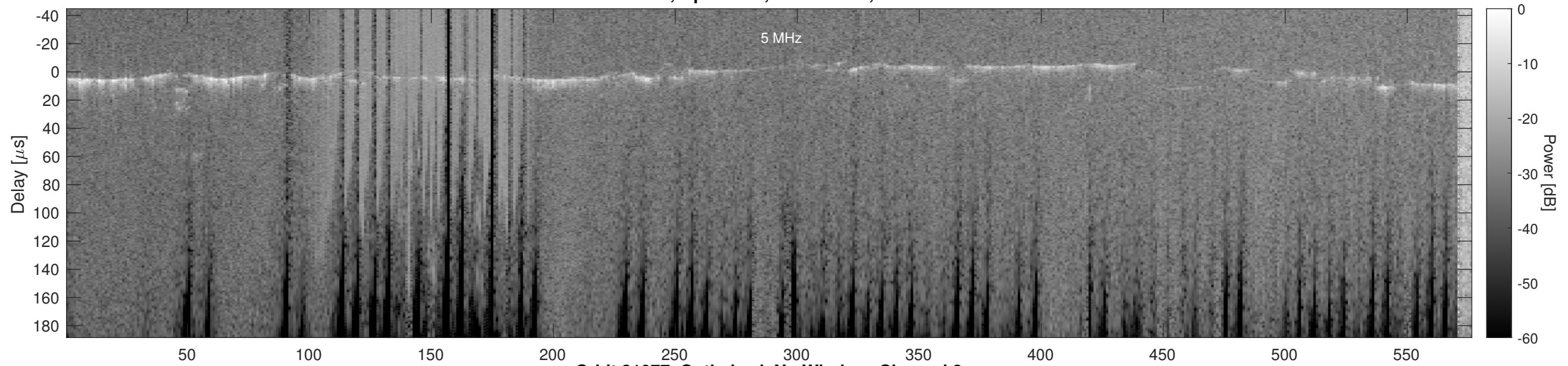
Orbit 21077, Optimized, No Window, Channel 2
