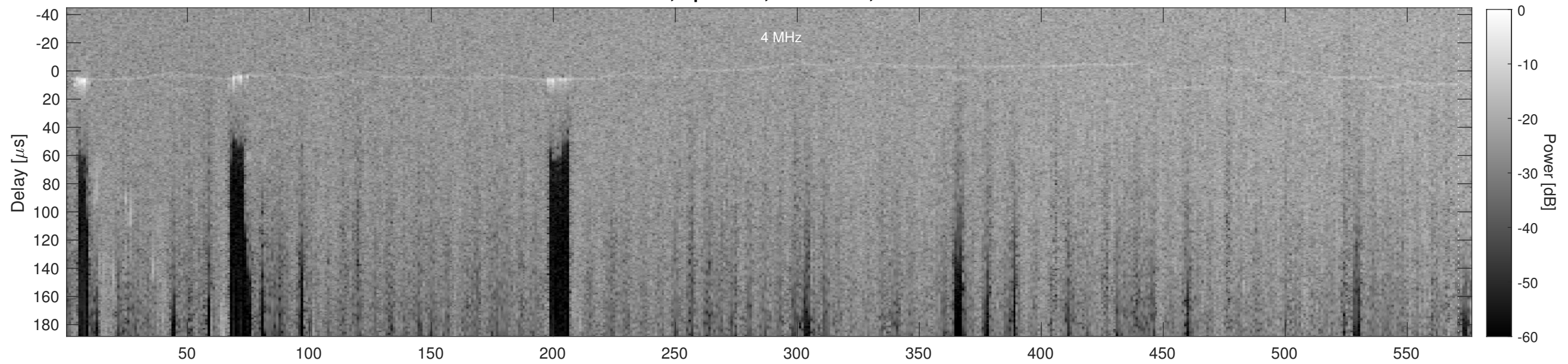
Orbit 21077, Cluttergram
