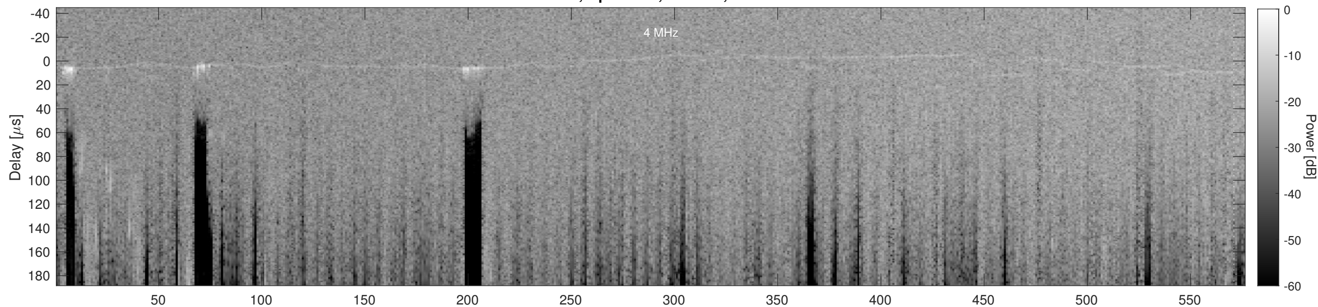
Orbit 21077, Cluttergram
