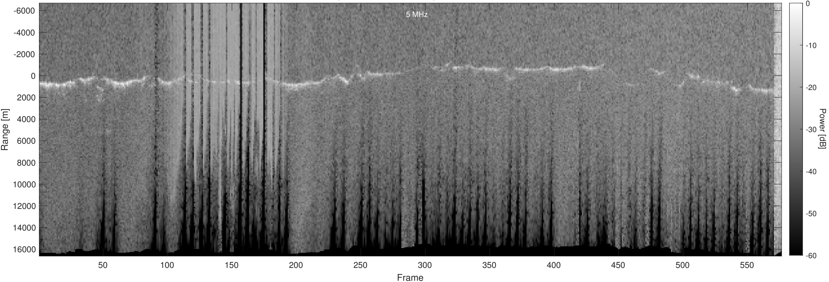
Orbit 21077, Optimized, Window, Depth-Corrected, Channel 2
