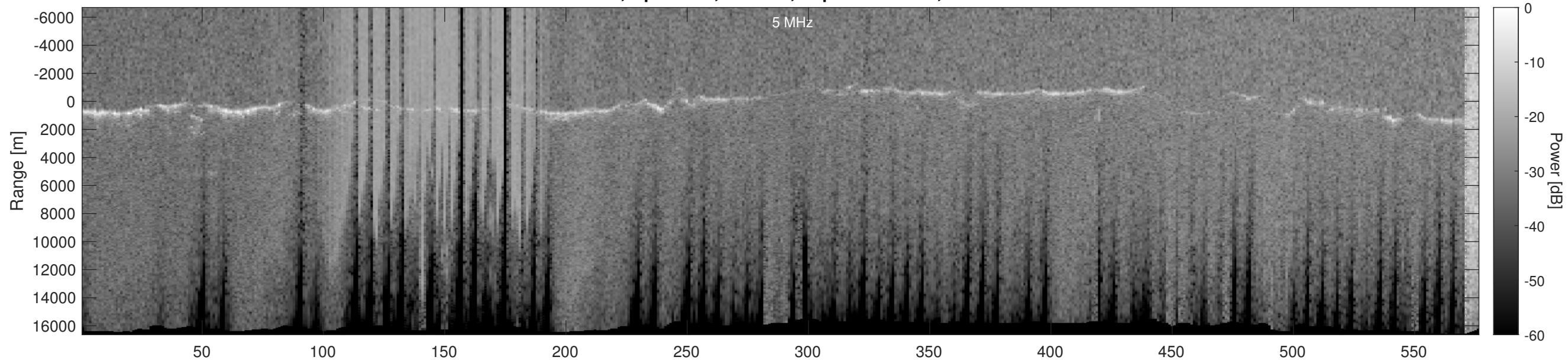
Orbit 21077, Optimized, Window, Depth-Corrected, Channel 2
