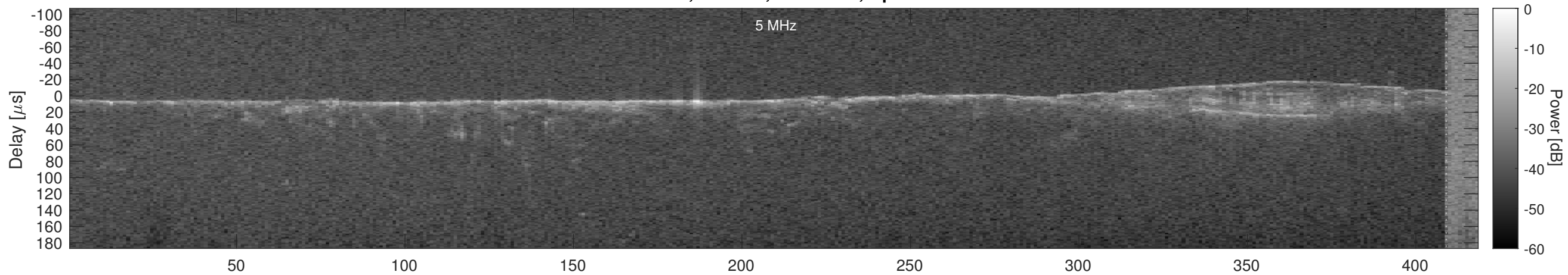
Orbit 21179, Cluttergram
