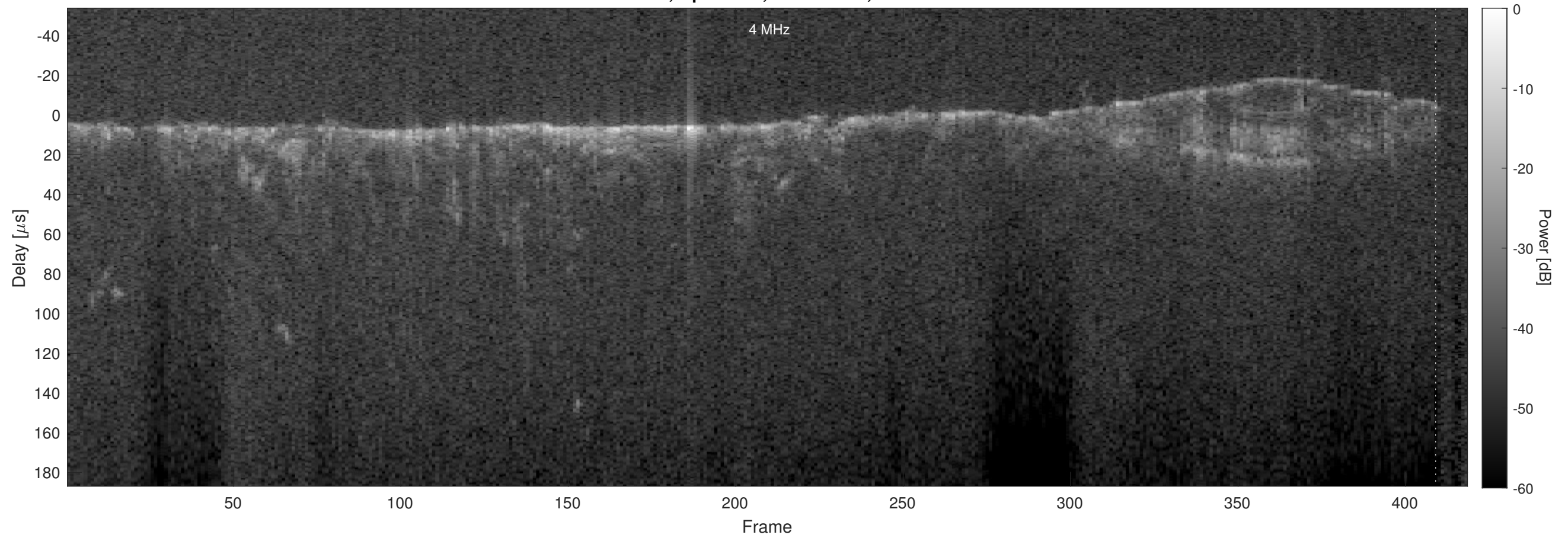
Orbit 21179, Optimized, No Window, Channel 2
