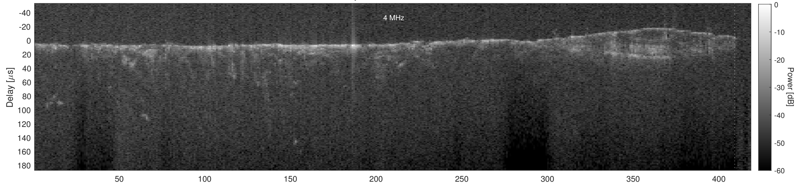
Orbit 21179, Cluttergram
