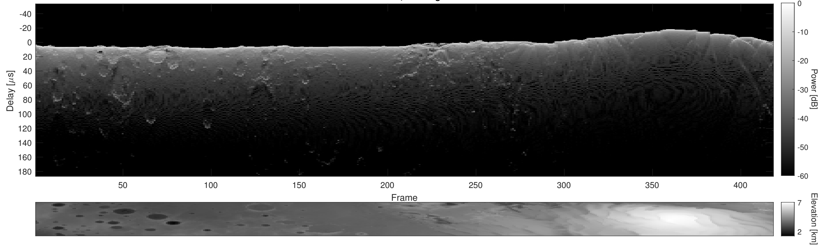
Orbit 21179, Cluttergram
