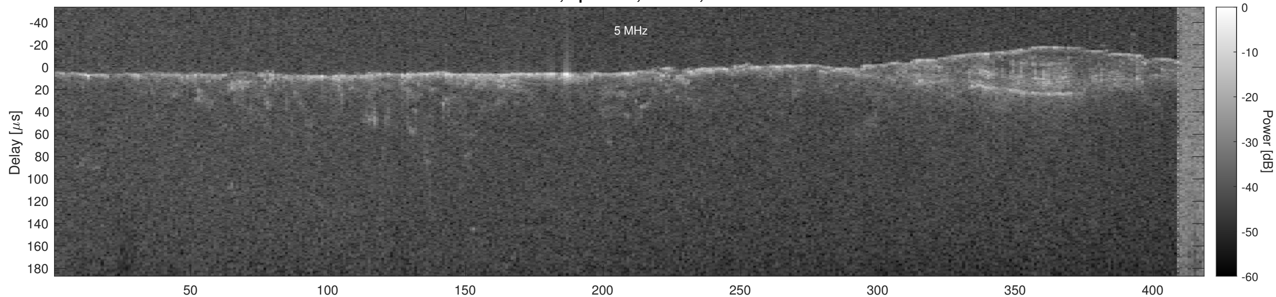
Orbit 21179, Optimized, Window, Channel 2
