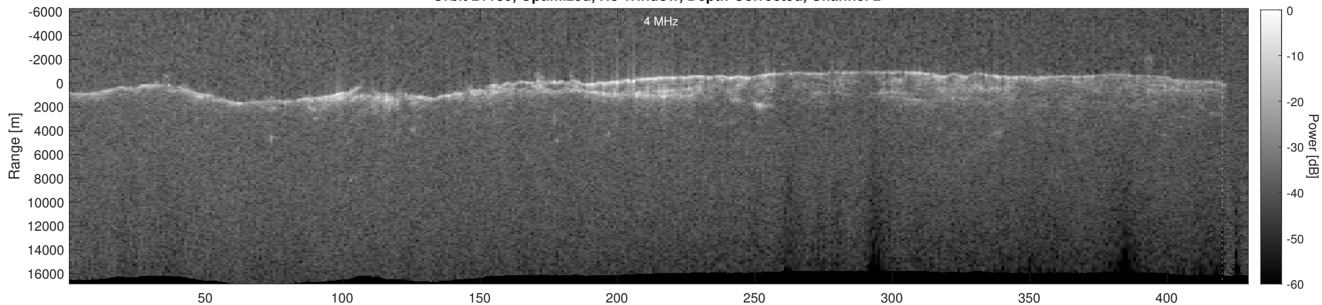
Orbit 21180, Depth-Corrected Cluttergram
