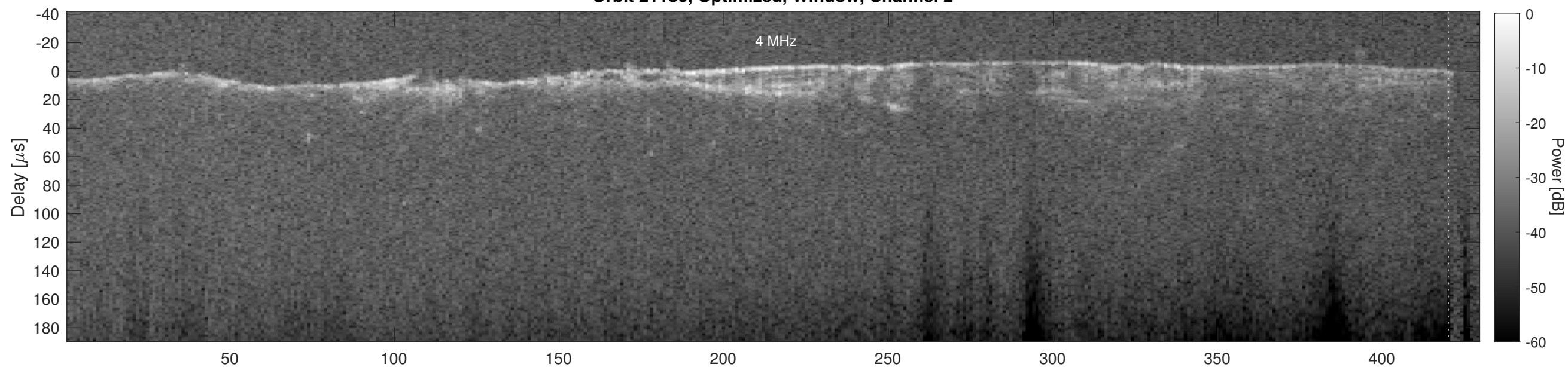
Orbit 21180, Cluttergram
