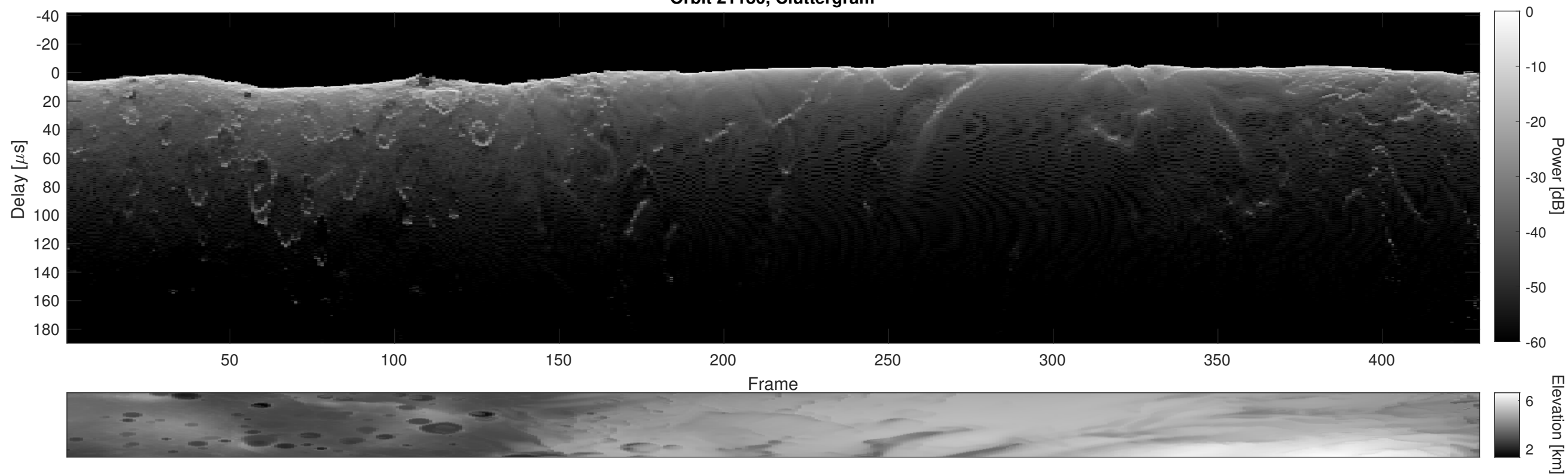
Orbit 21180, Cluttergram
