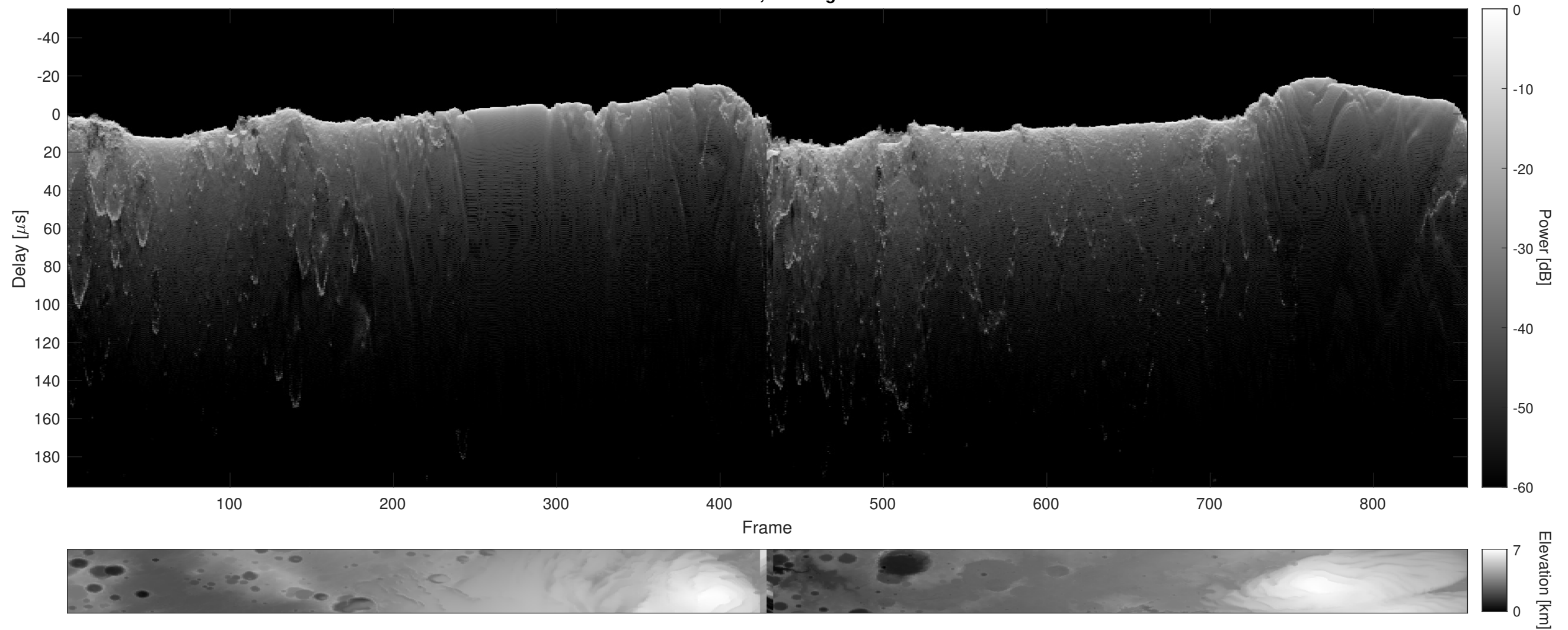
Orbit 21183, Cluttergram
