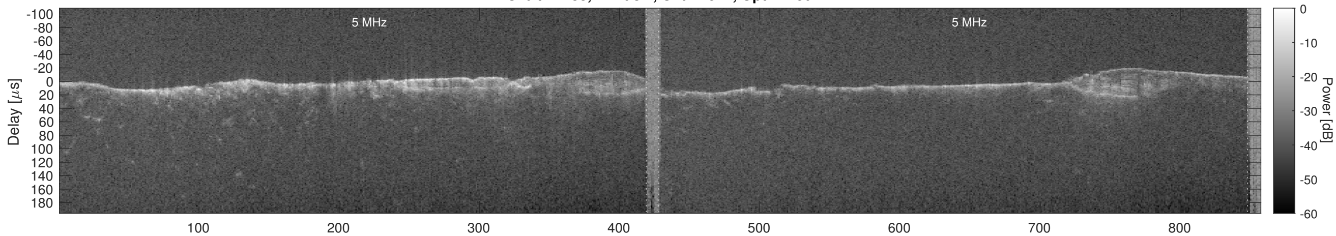
Orbit 21183, Cluttergram
