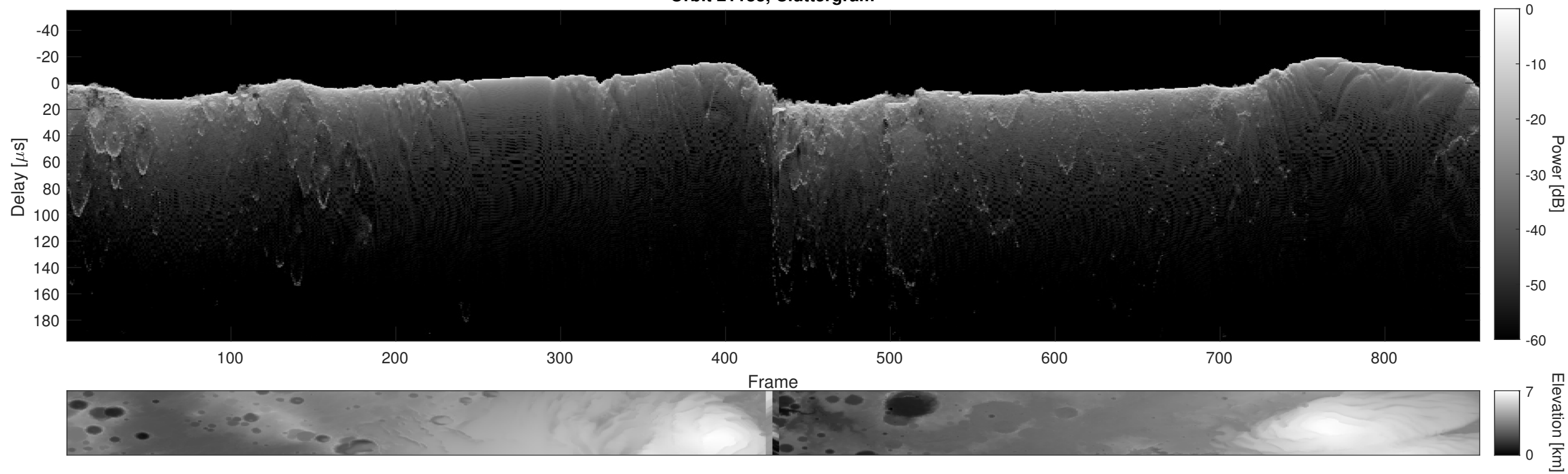
Orbit 21183, Cluttergram
