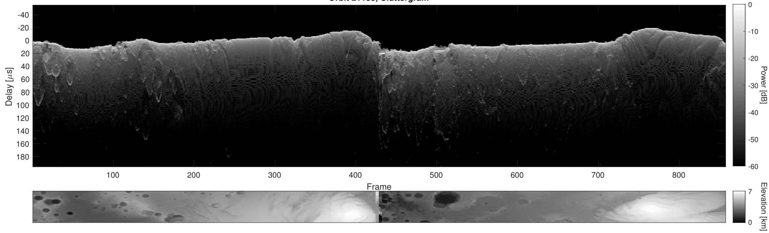
Orbit 21183, Cluttergram
