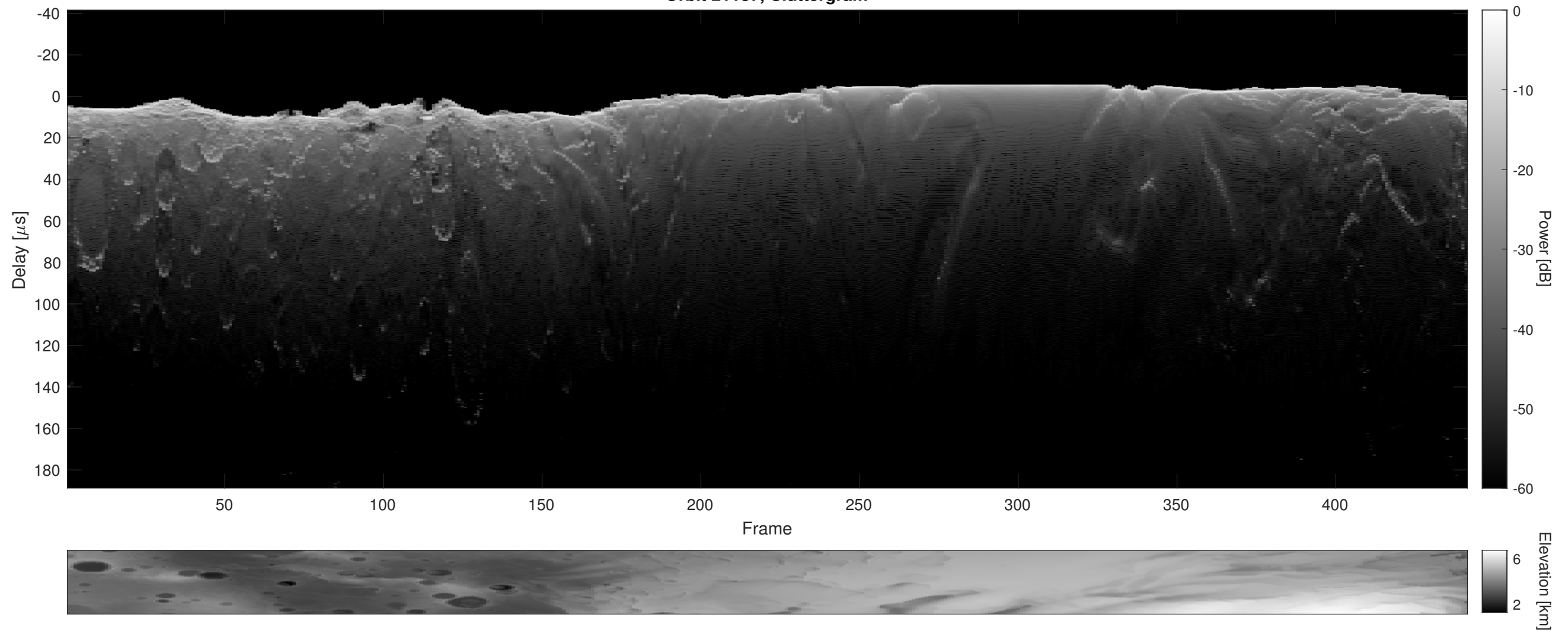
Orbit 21187, Cluttergram
