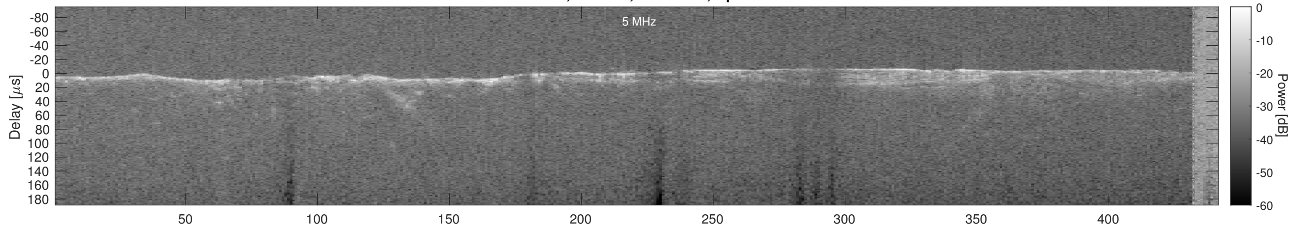
Orbit 21187, Cluttergram
