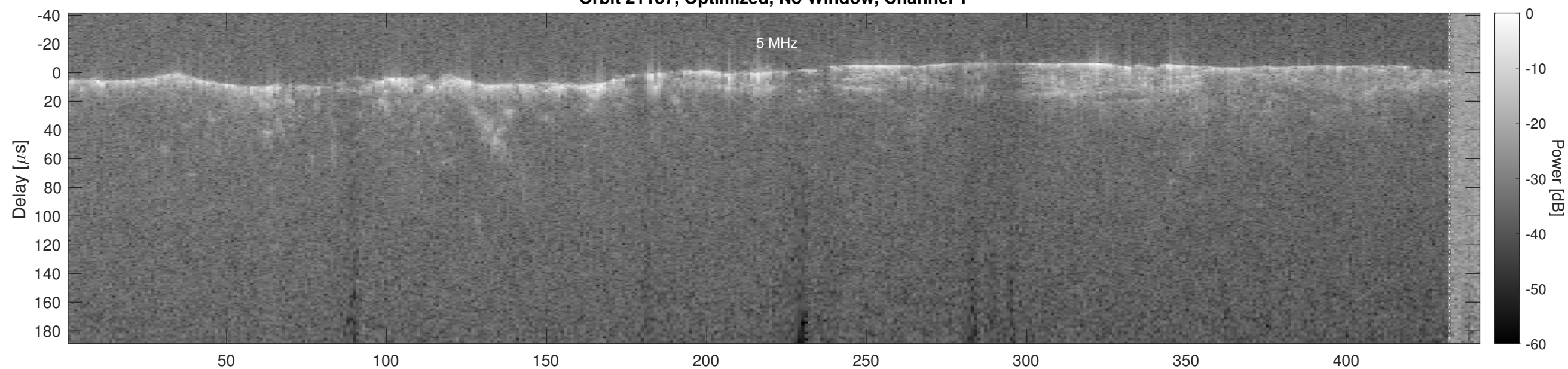
Orbit 21187, Optimized, No Window, Channel 2
