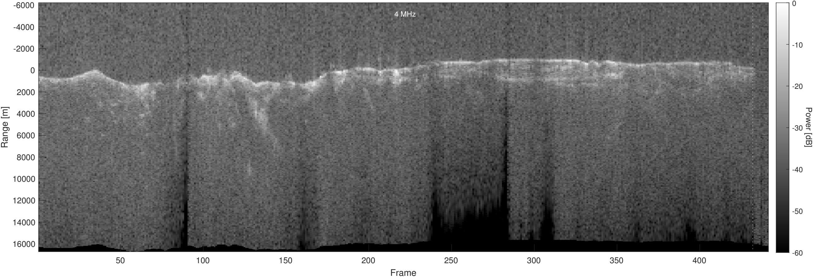
Orbit 21187, Optimized, No Window, Depth-Corrected, Channel 2
