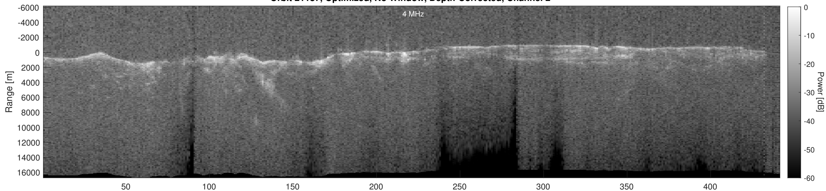
Orbit 21187, Depth-Corrected Cluttergram
