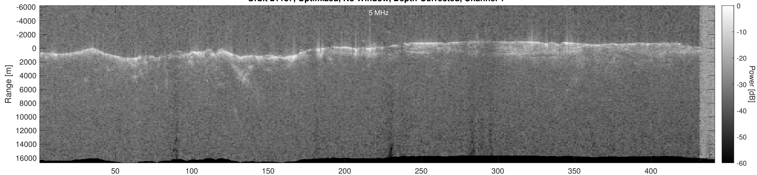
Orbit 21187, Optimized, No Window, Depth-Corrected, Channel 2
