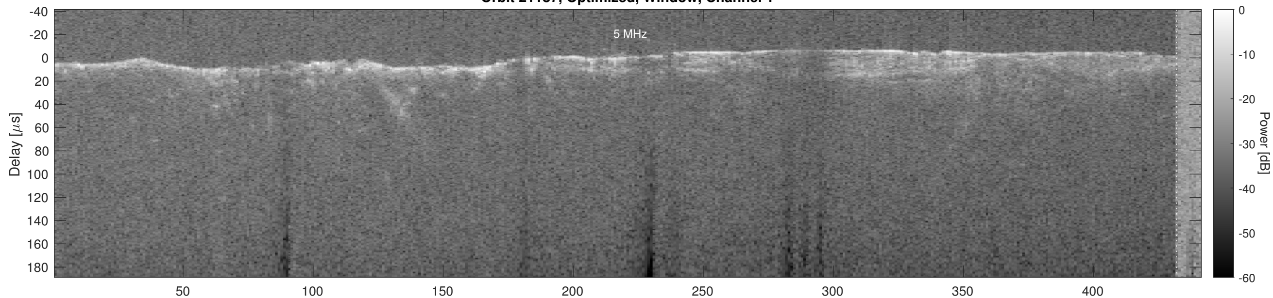
Orbit 21187, Optimized, Window, Channel 2
