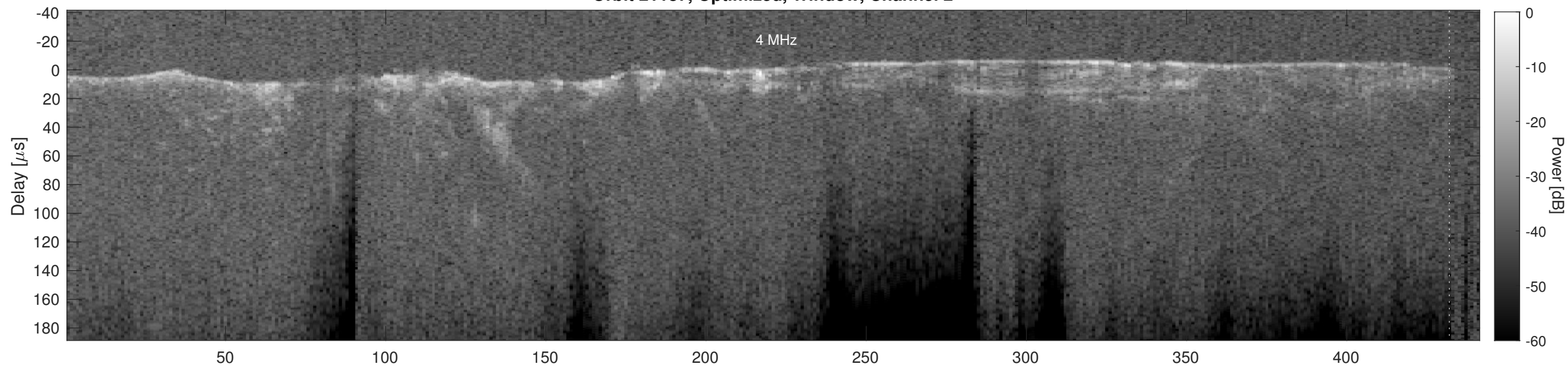
Orbit 21187, Cluttergram
