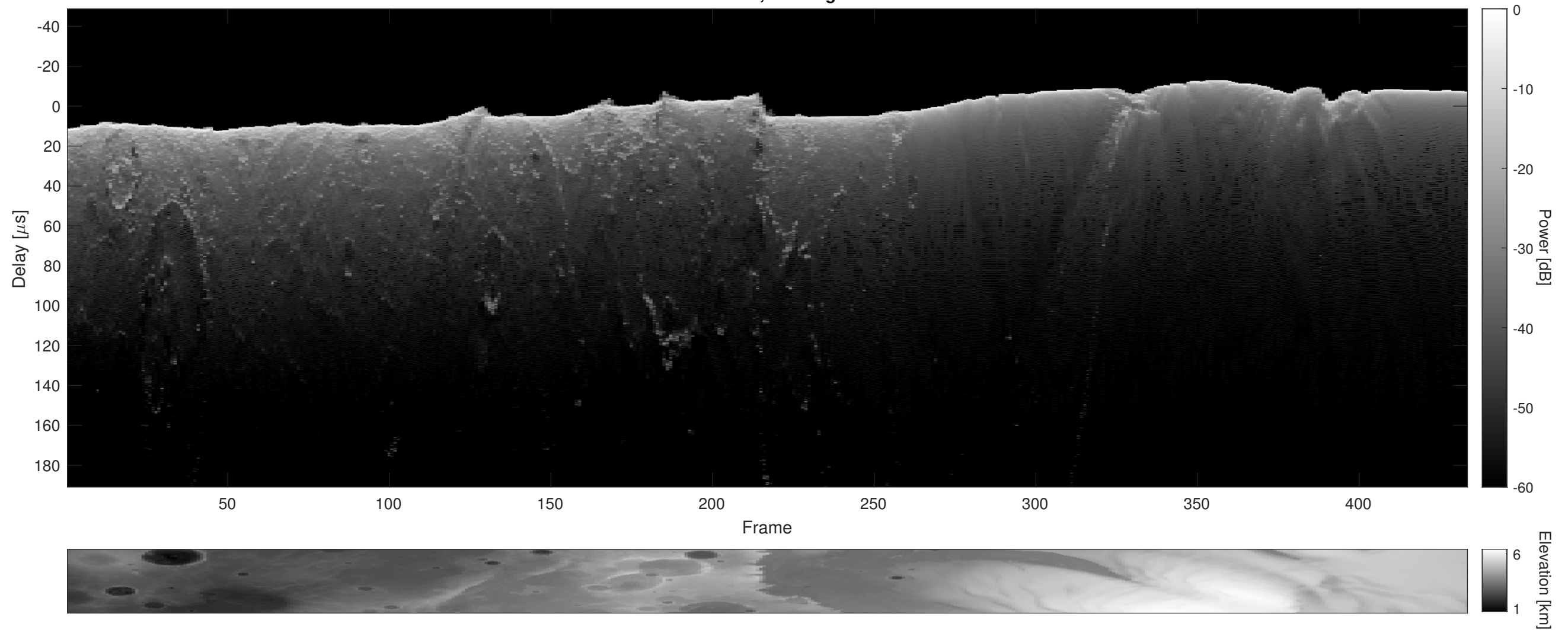
Orbit 21188, Cluttergram
