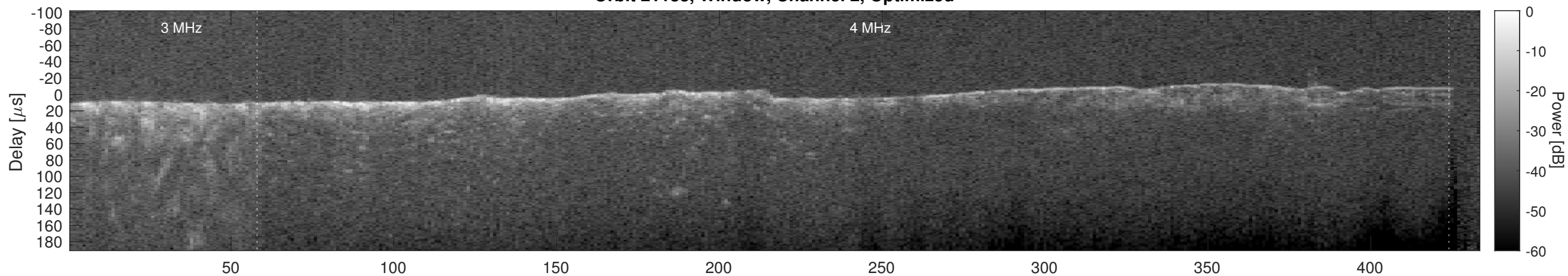
Orbit 21188, Cluttergram
