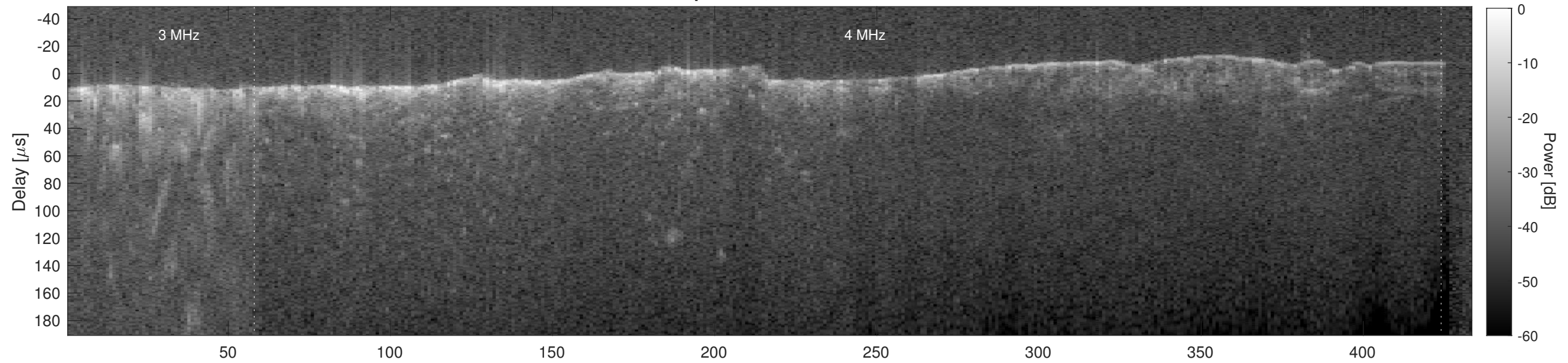
Orbit 21188, Cluttergram
