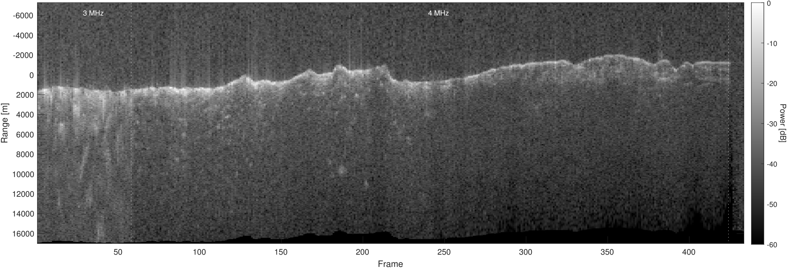
Orbit 21188, Optimized, No Window, Depth-Corrected, Channel 2
