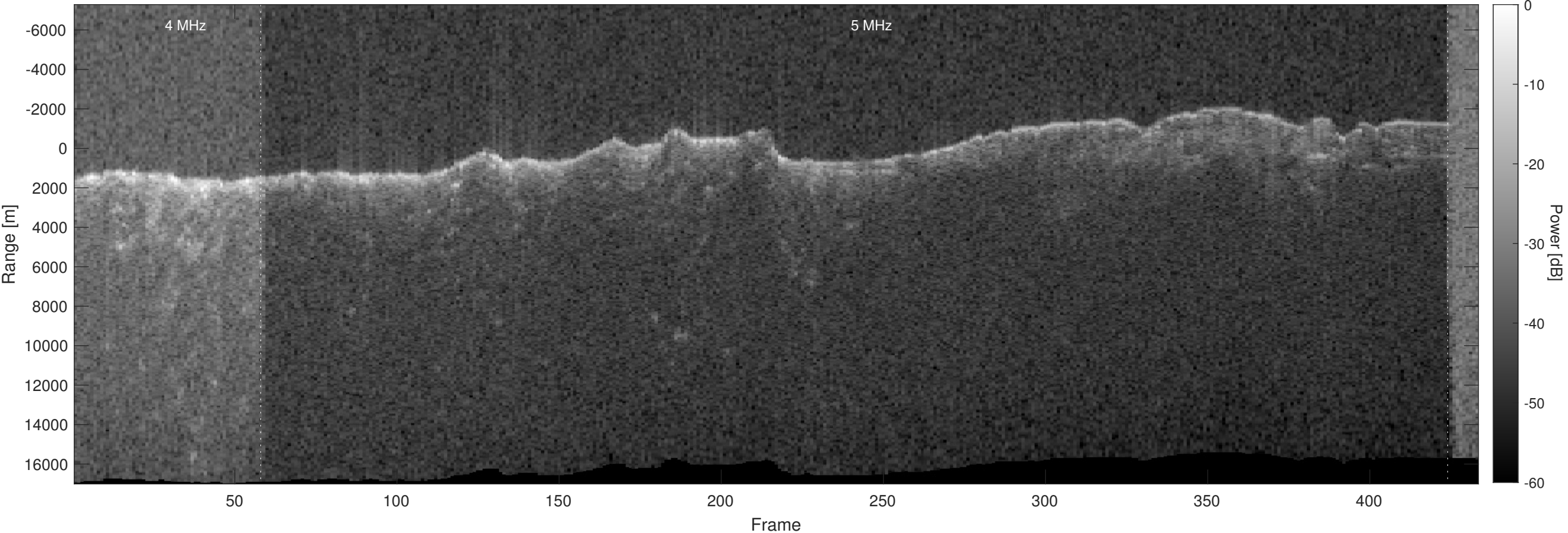
Orbit 21188, Optimized, Window, Depth-Corrected, Channel 2
