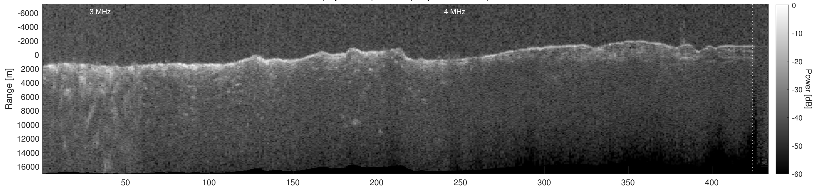
Orbit 21188, Depth-Corrected Cluttergram
