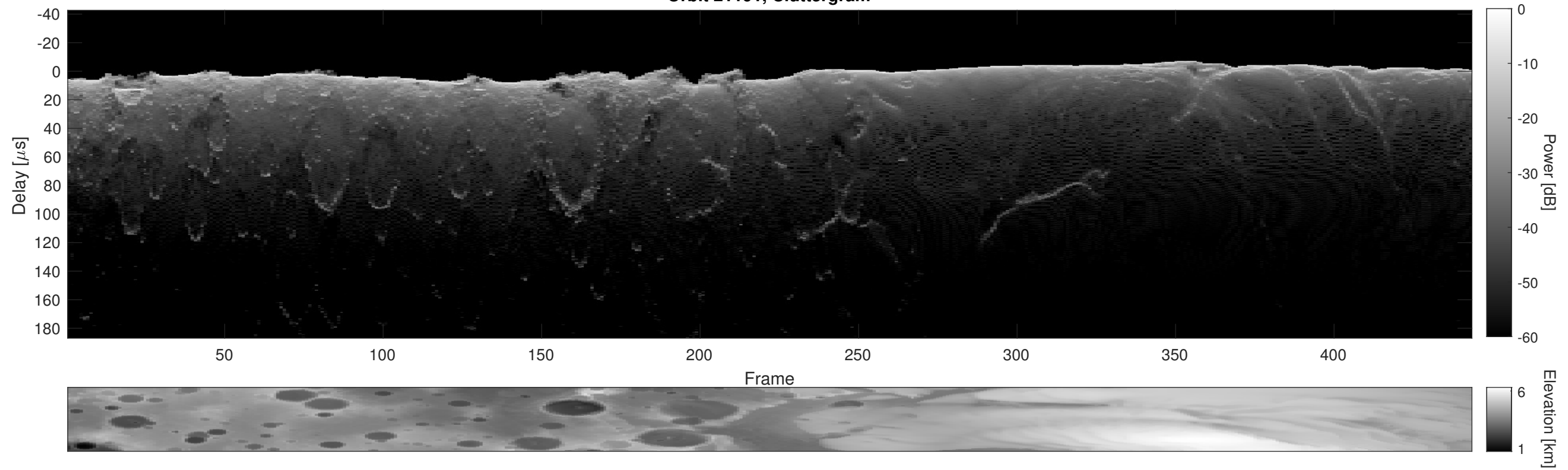
Orbit 21191, Cluttergram
