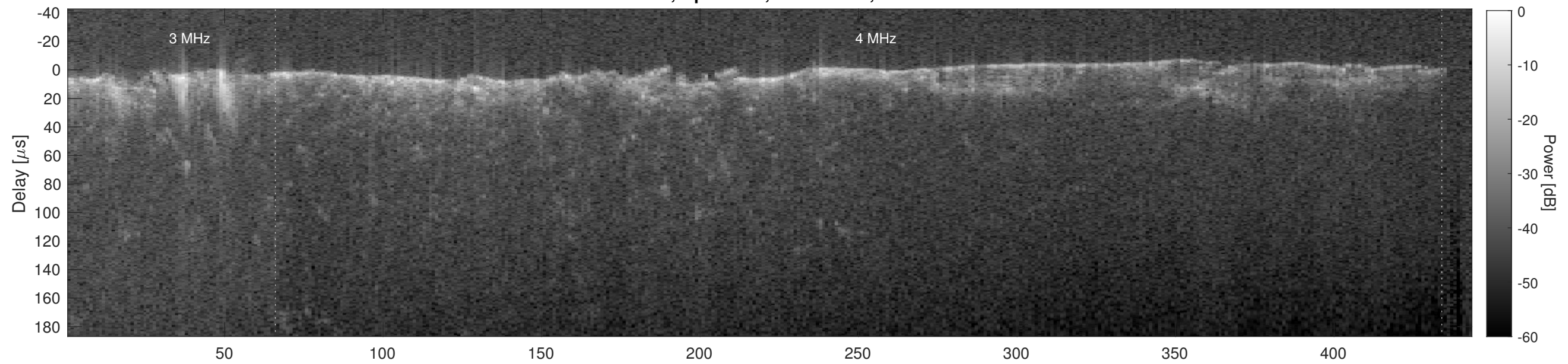
Orbit 21191, Cluttergram
