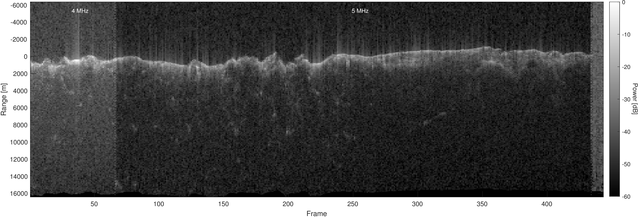
Orbit 21191, Optimized, No Window, Depth-Corrected, Channel 2
