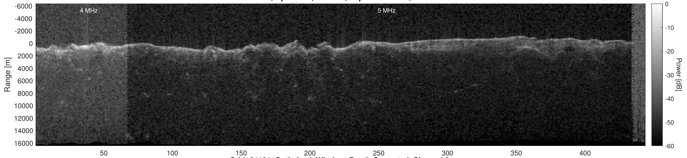
Orbit 21191, Optimized, Window, Depth-Corrected, Channel 2
