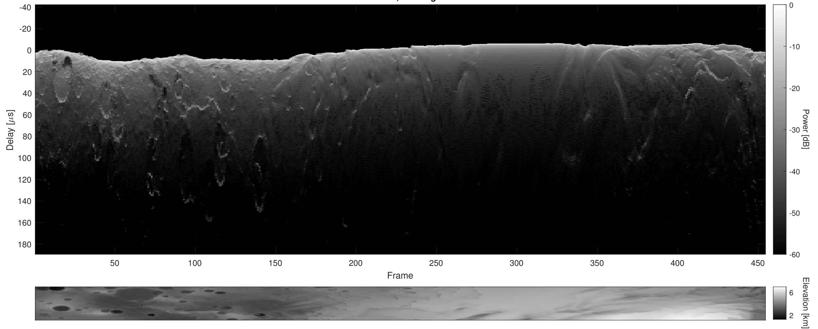
Orbit 21194, Cluttergram
