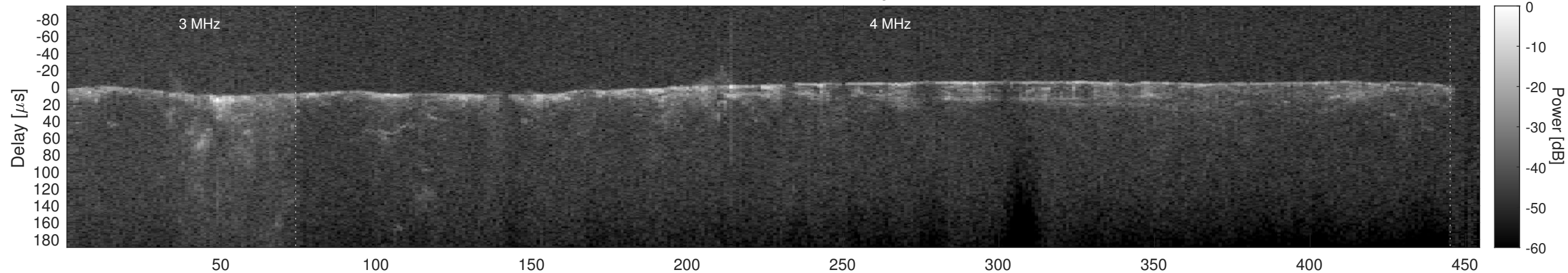
Orbit 21194, Cluttergram
