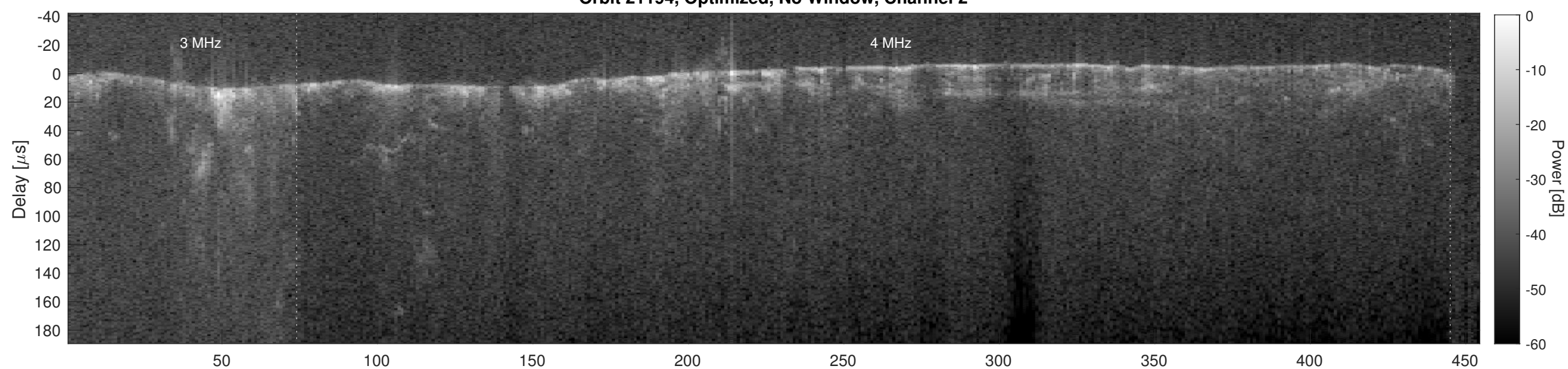
Orbit 21194, Cluttergram
