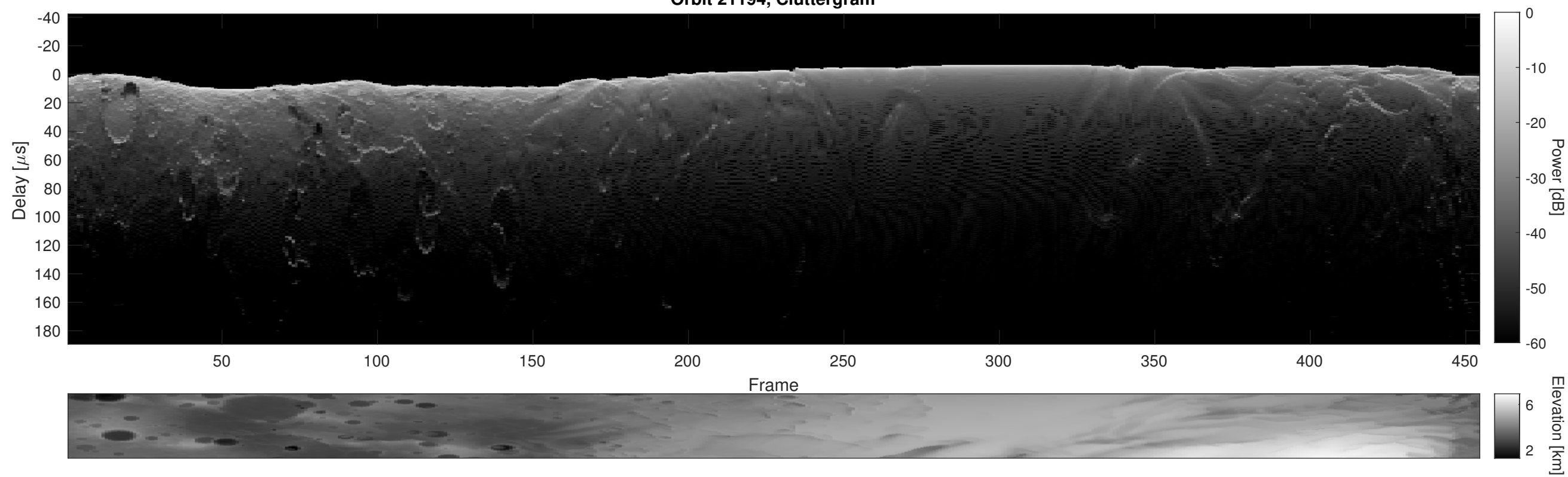
Orbit 21194, Cluttergram
