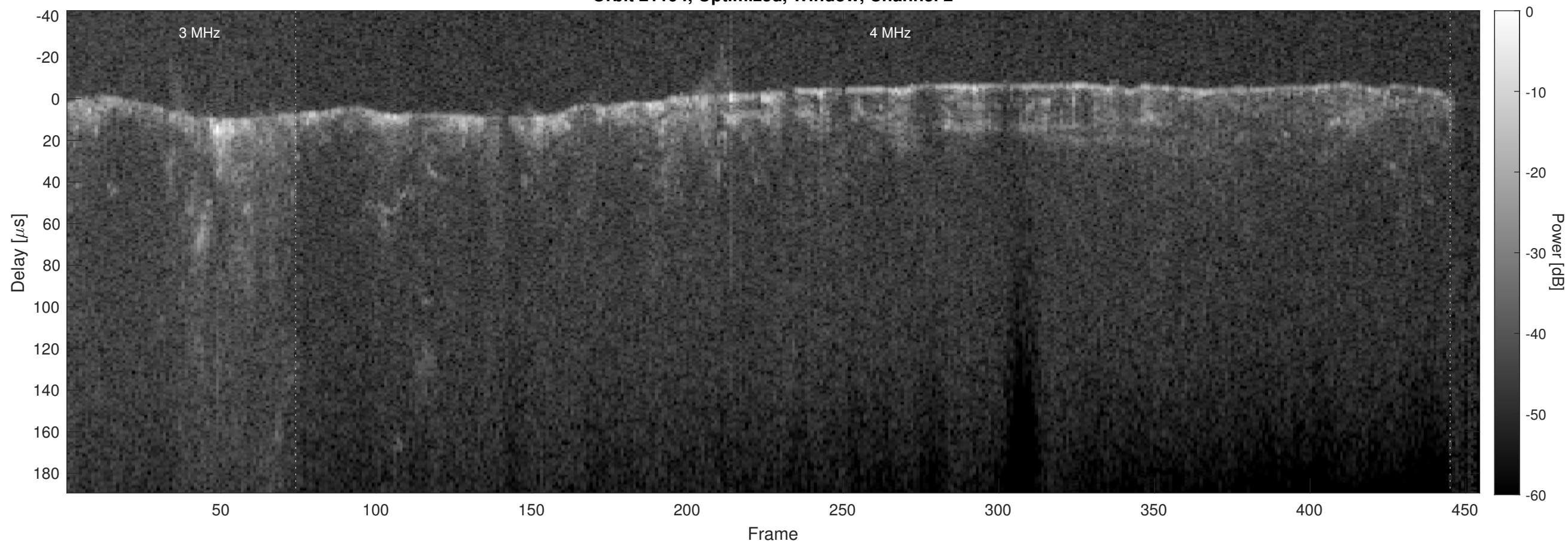
Orbit 21194, Optimized, Window, Channel 2
