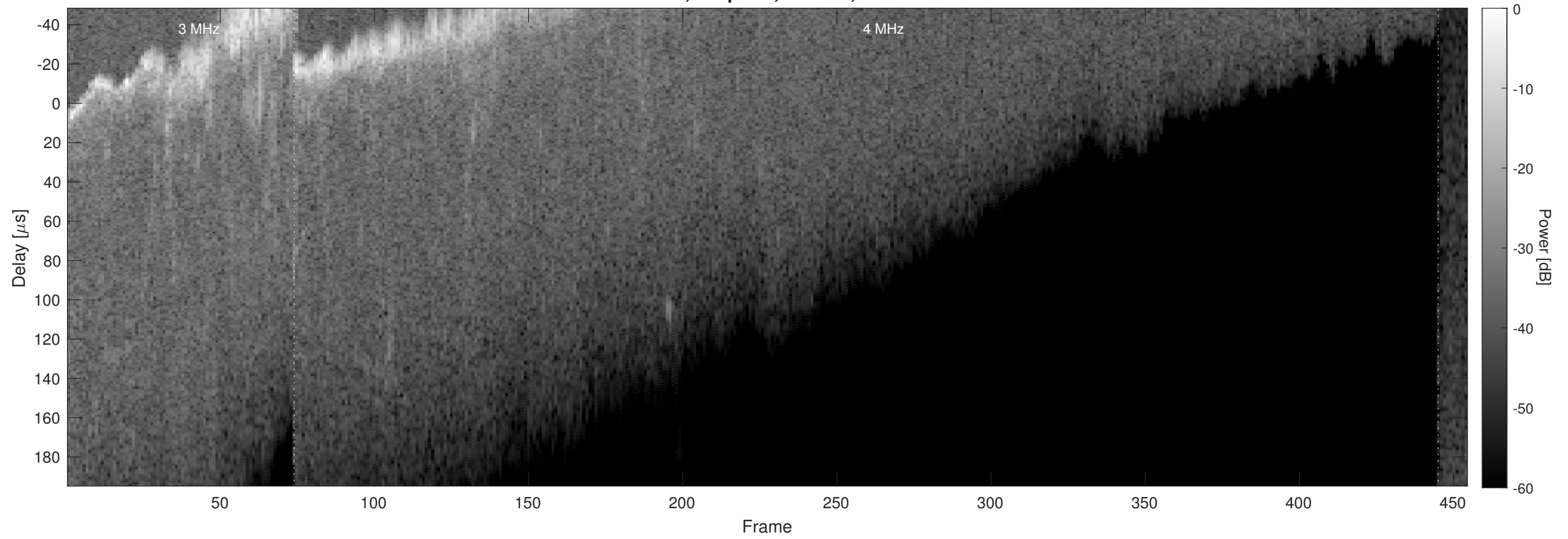
Orbit 21195, Chapman, Window, Channel 2
