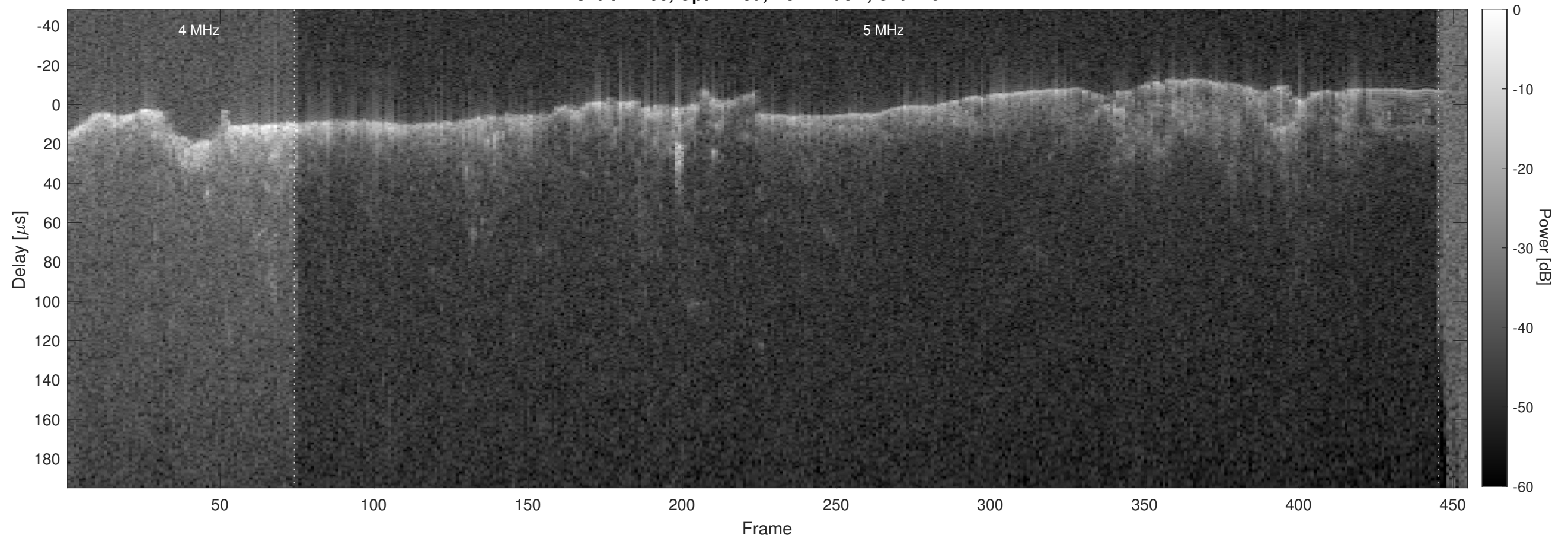
Orbit 21195, Optimized, No Window, Channel 2
