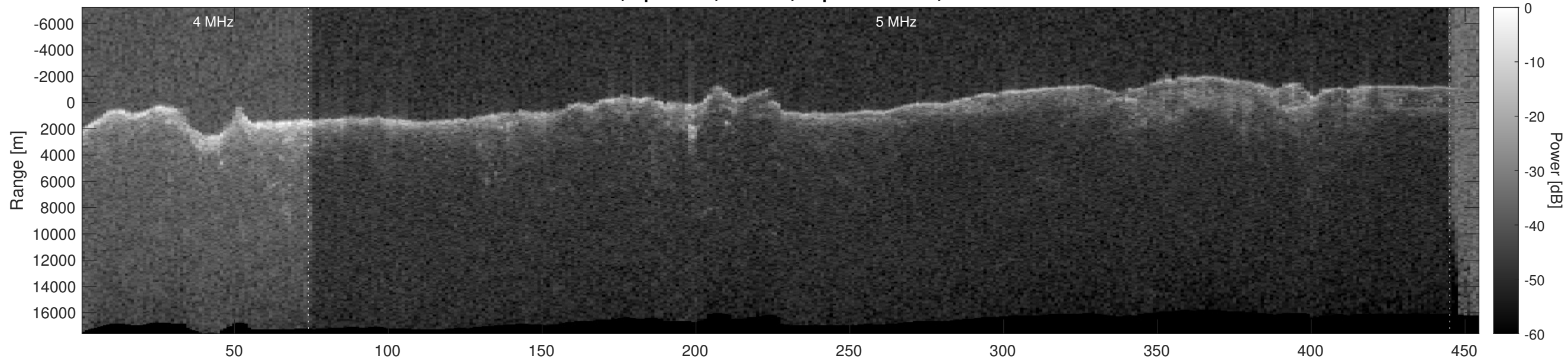
Orbit 21195, Optimized, Window, Depth-Corrected, Channel 2
