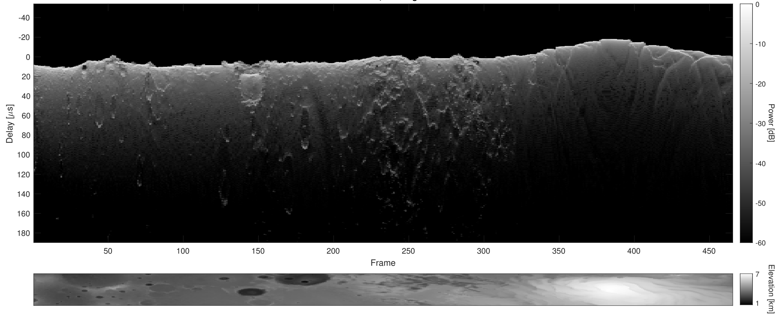
Orbit 21200, Cluttergram
