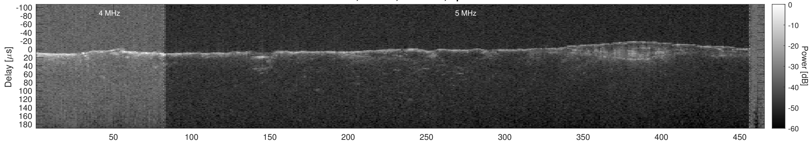
Orbit 21200, Cluttergram
