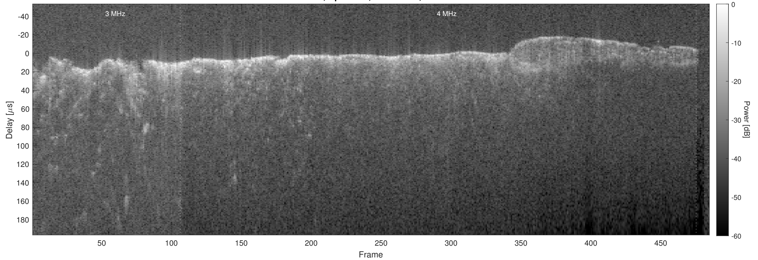
Orbit 21210, Optimized, No Window, Channel 2
