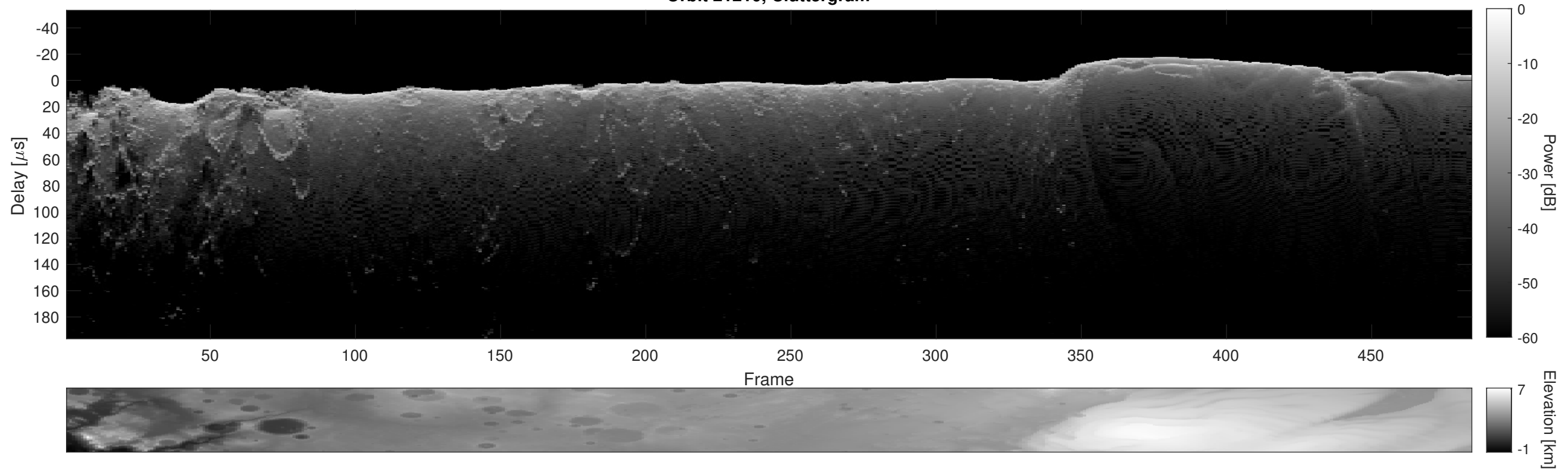
Orbit 21210, Cluttergram
