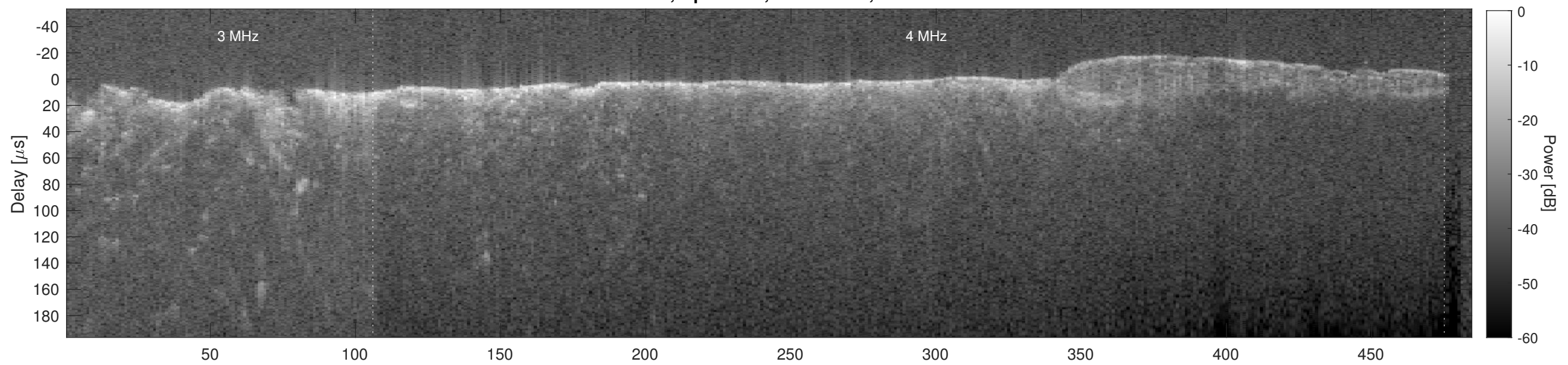
Orbit 21210, Cluttergram
