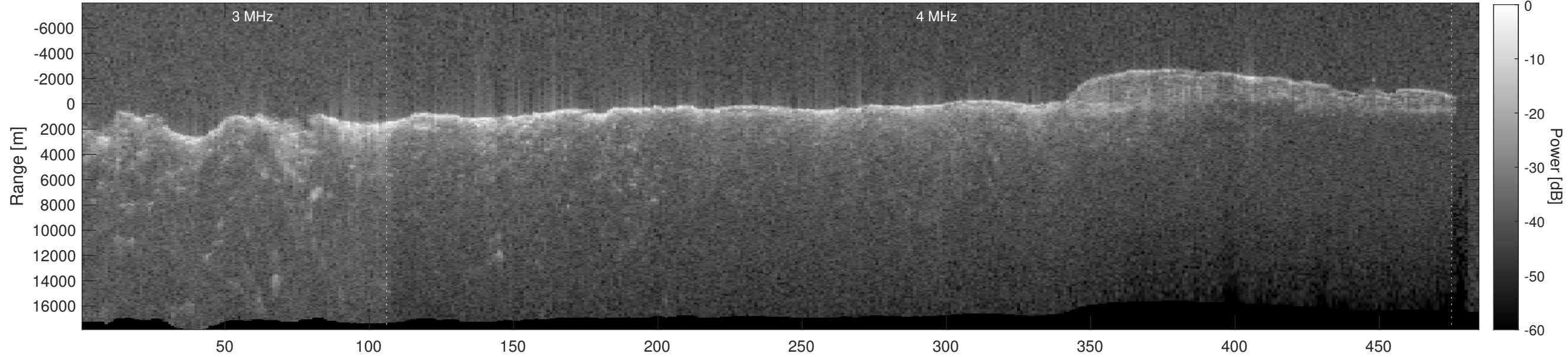
Orbit 21210, Depth-Corrected Cluttergram
