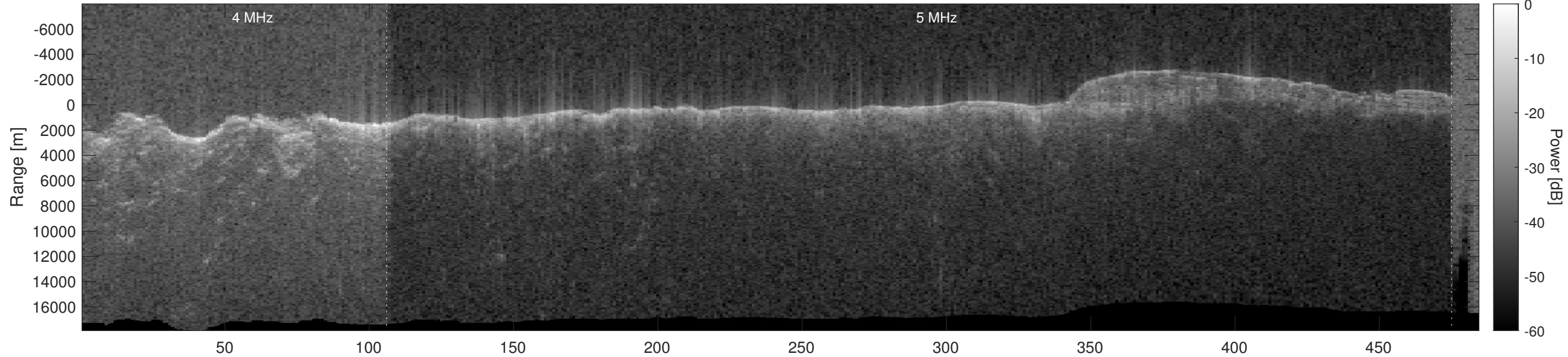
Orbit 21210, Optimized, No Window, Depth-Corrected, Channel 2
