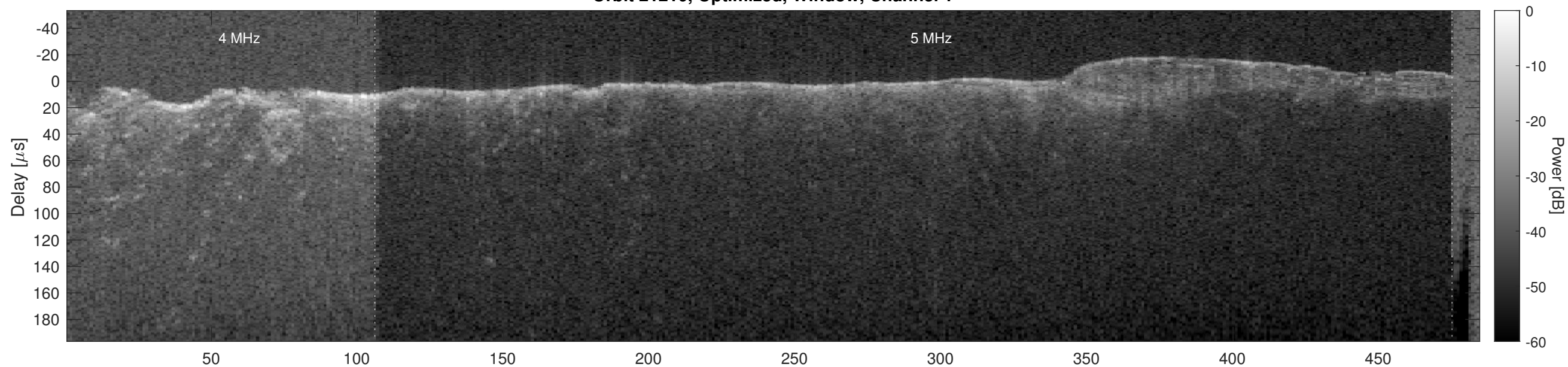
Orbit 21210, Optimized, Window, Channel 2
