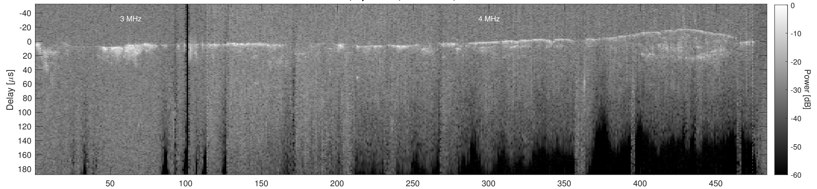
Orbit 21211, Cluttergram
